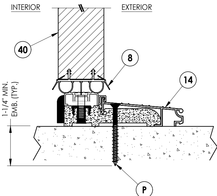
1 10 VERTICAL CROSS SECTION Inswing Sill
