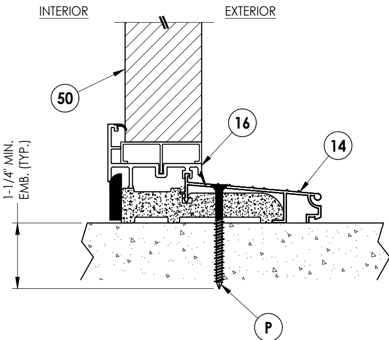
3 10 VERTICAL CROSS SECTION Inswing Sill
