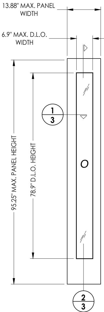
50 FIBERGLASS SIDELITE PANEL ODL FLUSH GLAZED
