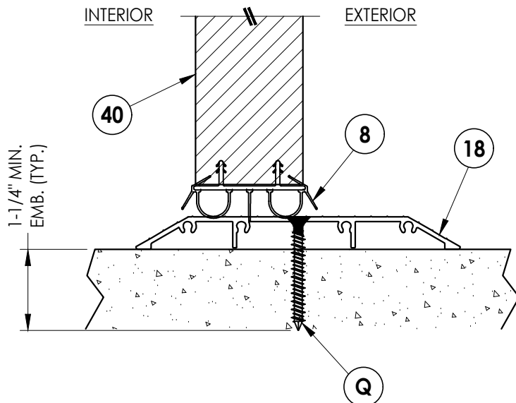
5 10 VERTICAL CROSS SECTION ADA Sill
